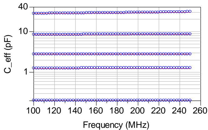
Legend: — Red solid lines - Model response on 60 mil Rogers 4003 ○ Blue symbols - Measurement on 60 mil Rogers 4003
