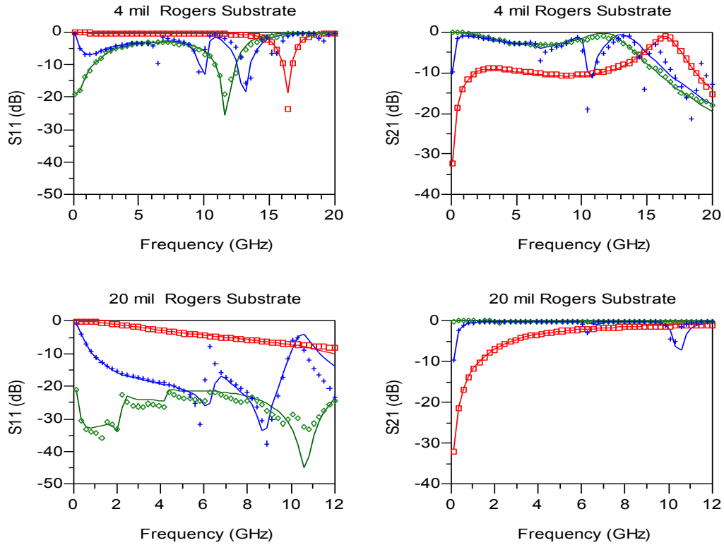
Legend: □ 0.4 pF, + 5.6 pF, ◇ 180 pF, Solid lines - Model data, Symbols - Measured data
