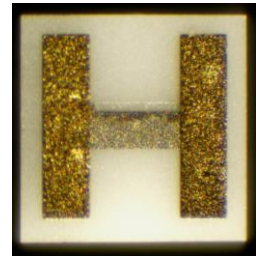
20x20 100Ω Microwave Resistor
