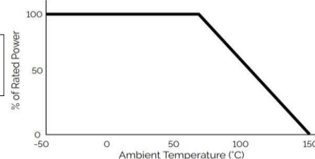
Power Derating Curve
