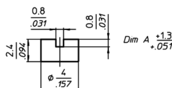
Figure B Order #: PPI-60-0410....-019 Slotted Sealcap Unmounted
