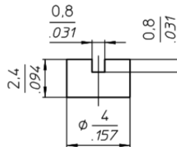
-019 Slotted Sealcap unmounted Dim A: +1.3 +0.51
