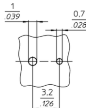
Mounting Layout
