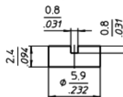
Figure B Order #: PPI-60-0609....-619 Slotted Sealcap Unmounted
