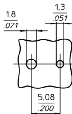
Mounting Layout
