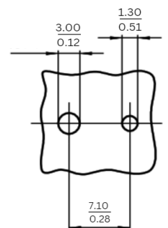
Mounting Layout
