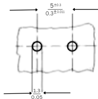
Installation Dimensions
